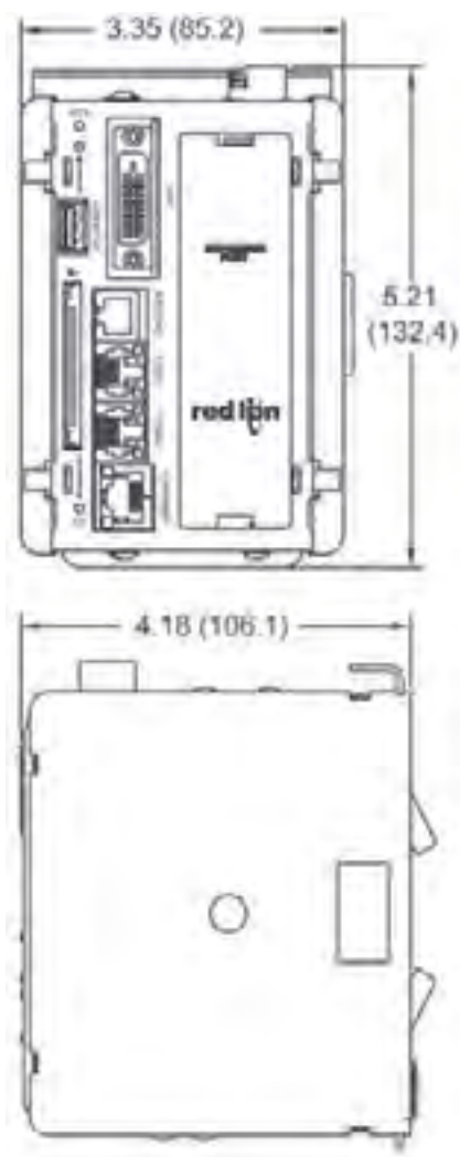
3.35" W x 5.21" H x 4.18" D (85.2mm W x 132.4mm H x 106.1mm D)
